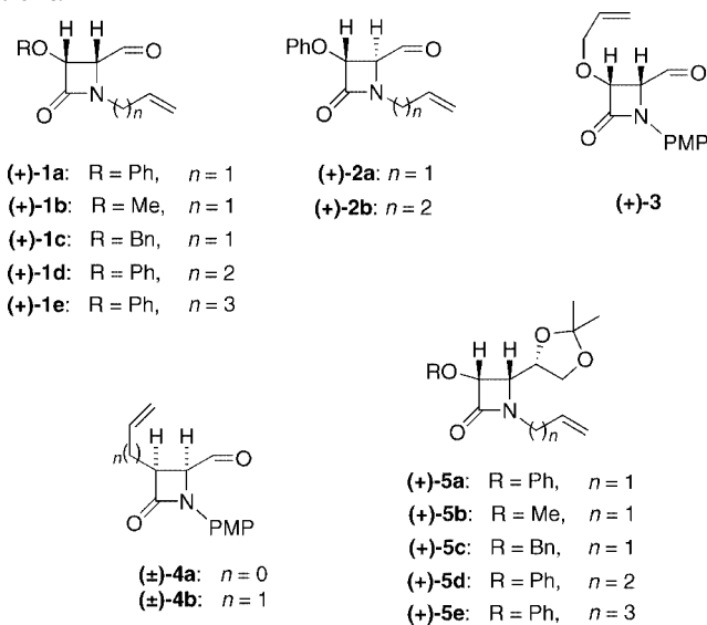
Figure 2. Starting 2-azetidinones 1–5 .
