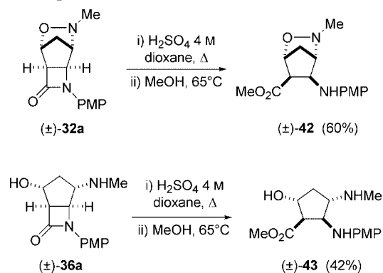
Scheme 15.
